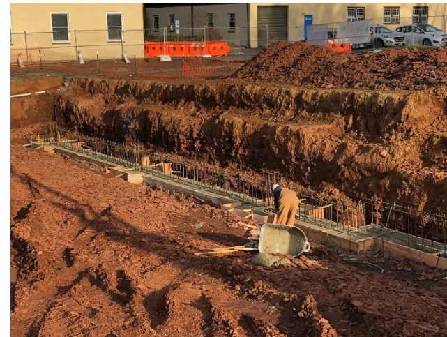
Continuing concrete for Municipal Building foundations
